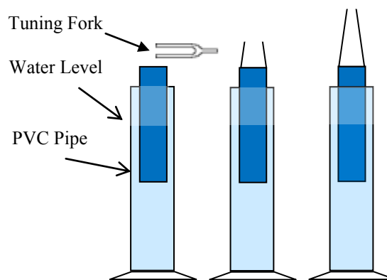
Figure 1 The range of situations that was investigated: from a cylindrical air column, to a cone topped tube with a small opening.
