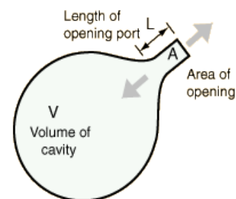
Figure 4 The length of a narrow opening of a classic Helmholtz resonator [2] .
